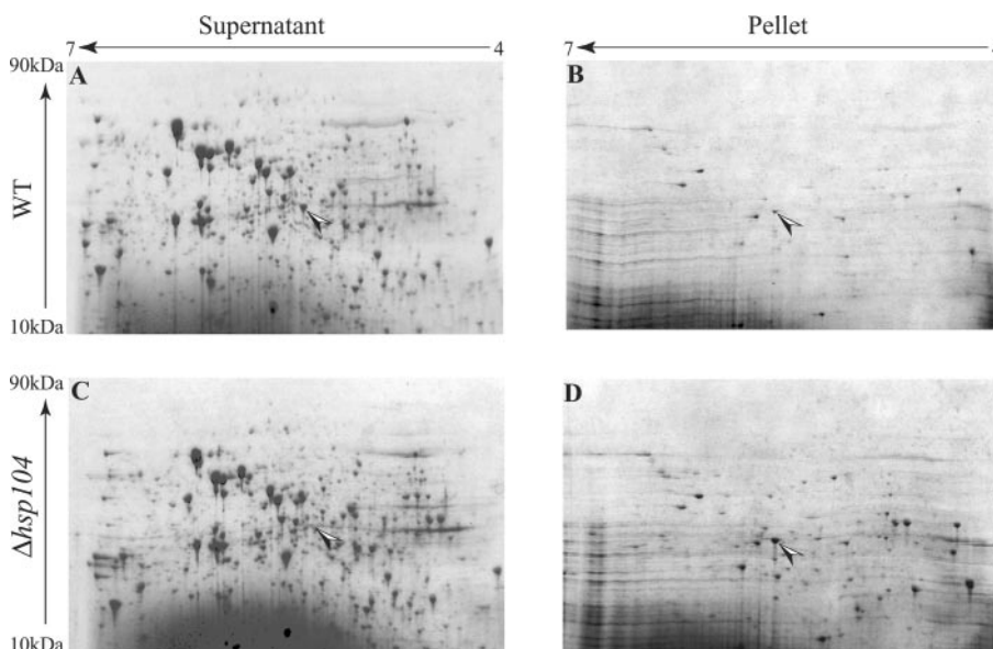
FIG. 1. Two-dimensional PAGE analysis of soluble and insoluble proteins after recovery from heat shock. Wild-type and hsp104 cells were pretreated at 37 °C for 30 min to induce the expression of heat shock proteins followed by a sublethal heat shock at 46 °C for 30 min. Protein synthesis was blocked by the addition of cycloheximide (10 \mu g/ml). The cells were allowed to recover at 25 °C for 2 h. Soluble and insoluble proteins were analyzed by two-dimensional PAGE. The spot corresponding to Hsp26 is marked with an arrow.
