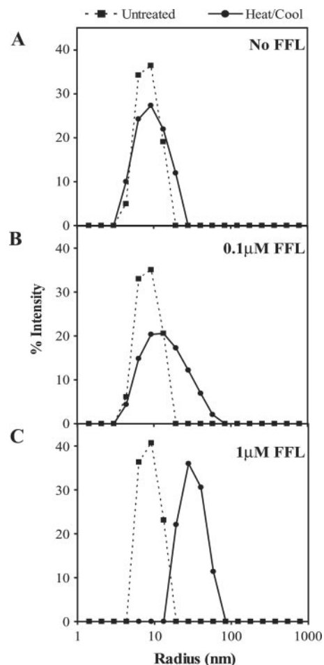
FIG. 6. Complex formation between Hsp26 and FFL monitored by dynamic light scattering. Samples were 0.42 \mu\text{M} Hsp26 oligomer ( A ), 0.42 \mu\text{M} Hsp26 oligomer with 0.1 \mu\text{M} FFL ( B ), and 0.42 \mu\text{M} Hsp26 oligomer with 1 \mu\text{M} FFL ( C ). Dotted line, untreated (25 ^{\circ}\text{C} ); solid line, heated at 45 ^{\circ}\text{C} for 10 s followed by cooling to 25 ^{\circ}\text{C} .
