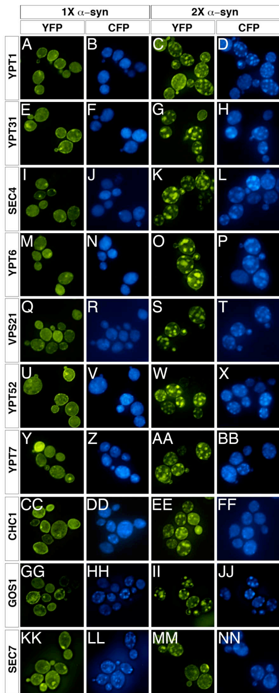
Fig. 3. \alpha -Syn perturbs Rab GTPase homeostasis. Fluorescence microscopy of 1 \times or 2 \times \alpha -syn-YFP-expressing cells in the presence of CFP-tagged Rab proteins. In 1 \times \alpha -syn cells (A, E, I, M, Q, U, Y, CC, GG, and KK), each CFP-Rab fusion localized properly based on published reports (B, F, J, N, R, V, and Z). In 2 \times \alpha -syn cells (C, G, K, O, S, W, and AA), each Rab was sequestered into the \alpha -syn inclusions (D, H, L, P, T, X, and BB). The localization of a CFP fusion to the clathrin heavy chain protein Chc1 (DD) was not altered in 2 \times \alpha -syn cells (EE and FF), indicating that the presence of a CFP tag was not responsible for the relocation of the Rab proteins. The Golgi vesicle-localized v-SNARE Gos1 (HH) colocalized with \alpha -syn inclusions (II and JJ), but Sec7p (KK and LL), an ARF GTP exchange factor, did not (MM and NN).
