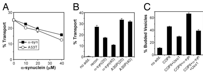
Fig. 1. \alpha -Syn accumulation inhibits in vitro ER→Golgi vesicular transport. (A) Reconstituted transport reactions in washed semiintact yeast cells containing [ ^{35} S]glyco-pro- \alpha -factor were incubated with increasing amounts of purified \alpha -syn or the \alpha -syn A53T variant. After 60 min at 25°C, the amount of Golgi-modified [ ^{35} S]glyco-pro- \alpha -factor was measured to determine transport efficiency. Transport in the absence of reconstitution factors was 2.4%, and plots represent levels minus this background. (B) In vitro reactions as in A comparing the influence of \alpha -syn and the A30P variant on reconstituted transport when added at 20 \mu M and 40 \mu M. (C) Semiintact cells as in A were incubated with COPII proteins or COPII plus Usol to measure budding and tethering in the presence or absence of \alpha -syn (40 \mu M). After 25 min at 25°C, freely diffusible vesicles containing [ ^{35} S]glyco-pro- \alpha -factor were separated from semiintact cells by centrifugation, and percentages of budded vesicles were determined.
