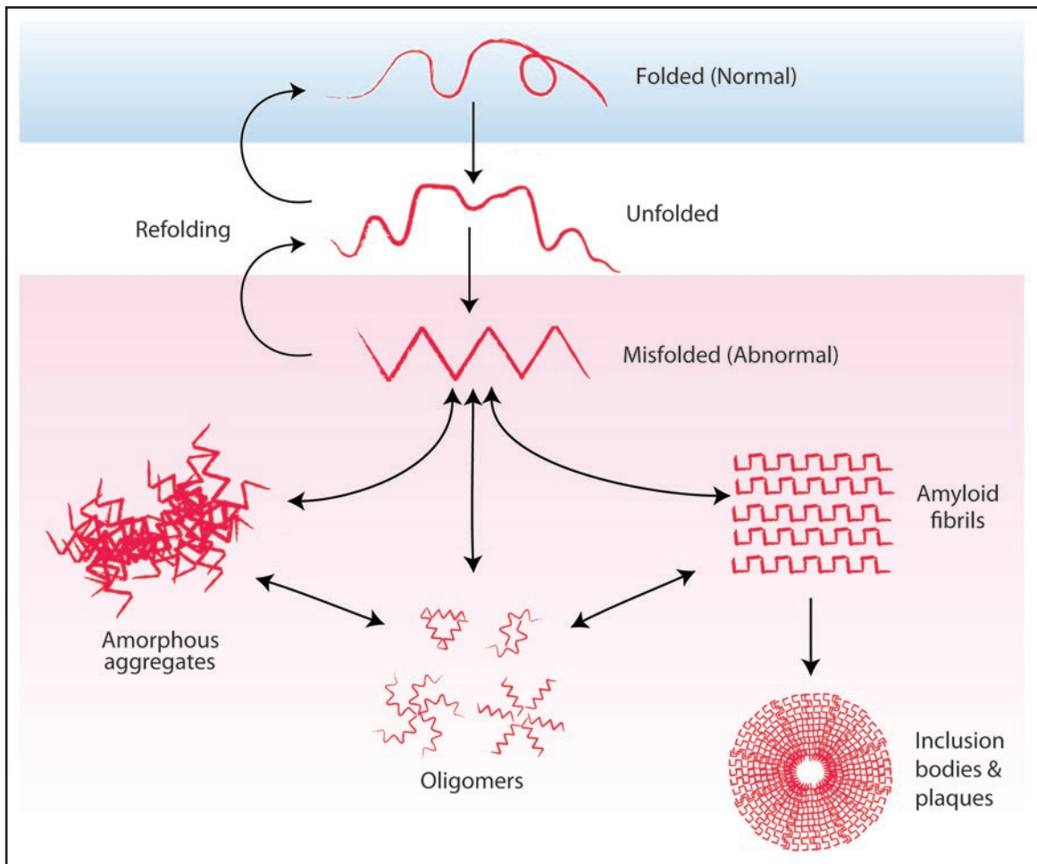
Figure 1. Aggregation of misfolded protein can give rise to oligomers, amorphous aggregates and inclusion bodies. The accumulation of misfolded protein leads to the formation of different protein assemblies. Prefibrillar oligomers formed by different proteins share a common structure and are thought to be the toxic protein species in diseases such as Alzheimer disease and Huntington disease. 5,6 Oligomers are conformationally molten and can associate to form amorphous aggregates or convert to an amyloidogenic nucleus to initiate amyloid fibril formation. Amyloid fibrils have a highly organized structure due to repeating \beta -sheets and are insoluble. Amyloid fibrils are often found in intra- and extracellular inclusions such as inclusion bodies and amyloid plaques. The generation of amyloid fibers and inclusion bodies can protect cells by reducing the formation of highly interactive toxic oligomers and amorphous aggregates.
