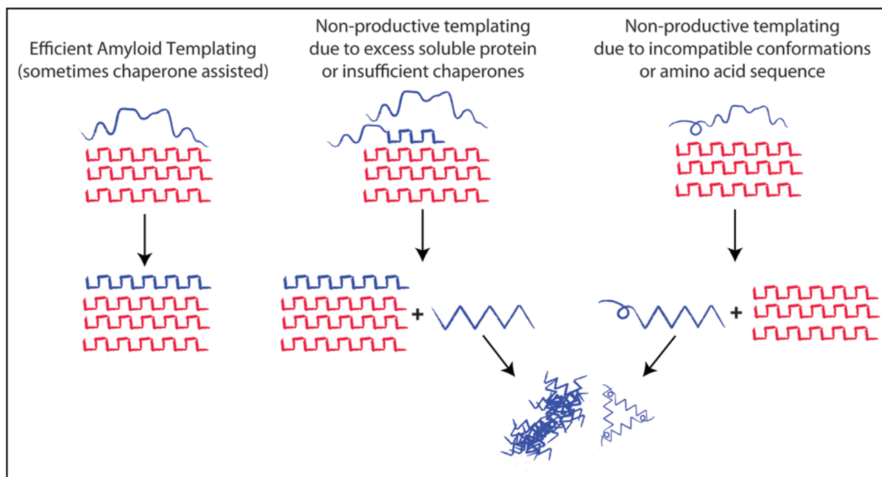
Figure 2. Amyloid and Non-productive templating. Amyloid fibrils grow by causing proteins of the same amino-acid sequence to adopt the same amyloid conformation. This is referred to as amyloid templating and involves the efficient addition of monomers or oligomeric species to the amyloid fiber, which may be assisted by specific chaperones (e.g., Rnq1 and the Hsp40 Sis1, Sup35NM and Hsp104, 49 ). If the amount of substrate exceeds the cellular capacity for amyloid conversion or if amino acid sequences are incompatible, the interaction of substrate with the amyloid fibrils may give rise to other abnormal conformational species, which may go on to form toxic oligomers and amorphous aggregates (Rnq1, PrP and Het-s/S). We refer to this as non-productive templating.
